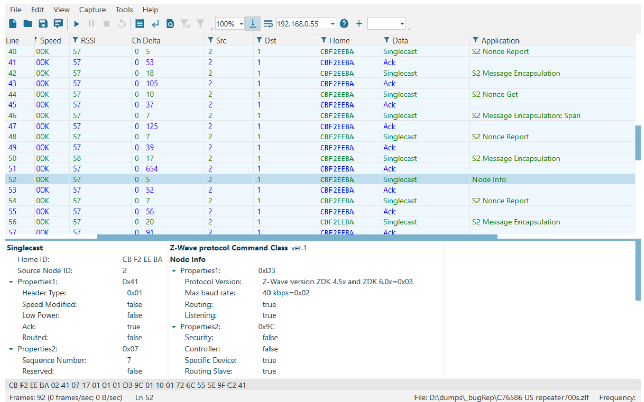
Figure 3. Z-Wave Zniffer Main Application Window
